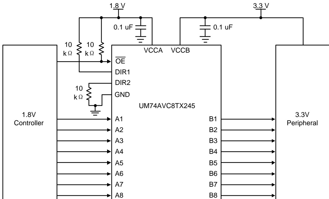
Figure 11-1. UM74AVC8TX245 Typical Application
